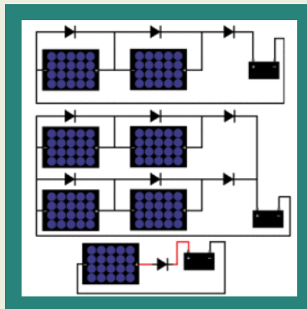
Diodes for Solar Applications
